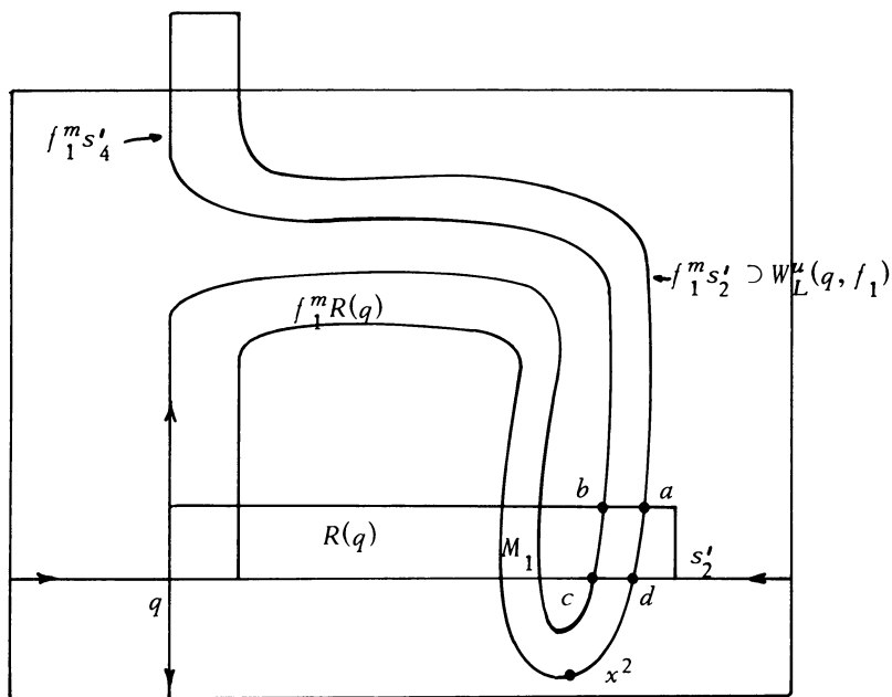
Figure 10. \tilde{F}(q, f_1)
