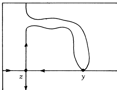
Figure 7. \tilde{F}_0(z)
